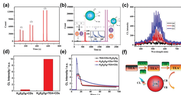
Fig. 10 (a) CL curves of a \text{KIO}_4-\text{H}_2\text{O}_2-\text{N} -doped CDs system ((1) \text{H}_2\text{O}_2 was added to the mixture of \text{KIO}_4 and N-CDs, (2) N-CDs was added to the mixture of \text{KIO}_4 and \text{H}_2\text{O}_2 , (3) \text{KIO}_4 was added to the mixture of \text{H}_2\text{O}_2 and N-CDs). (b) The mechanism of enhancement of the CL of the \text{KIO}_4-\text{H}_2\text{O}_2 system by N-doped CDs in acidic (the decreasing effect) and basic (increasing effect) solutions. (c) CL spectra of the \text{KIO}_4-\text{H}_2\text{O}_2 system in the presence and absence of N-doped CDs and NaOH (a: \text{KIO}_4-\text{H}_2\text{O}_2 , b: \text{KIO}_4-\text{H}_2\text{O}_2-\text{N} -doped CDs, c: \text{KIO}_4-\text{H}_2\text{O}_2-\text{N} -doped CDs-NaOH). 157 (Reprinted with permission from the American Chemical Society, Copyright 2016.) (d) The CL spectrum of the \text{CNDs}/\text{K}_2\text{S}_2\text{O}_8 system and the \text{CNDs}/\text{TEA}/\text{K}_2\text{S}_2\text{O}_8 system. (e) CL spectrum of the \text{CNDs}/\text{TEA}/\text{K}_2\text{S}_2\text{O}_8 system under different reagent mixing orders. (f) The scheme of the CL mechanism of the \text{CNDs}/\text{K}_2\text{S}_2\text{O}_8/\text{TEA} system. 158 (Reprinted with permission from the American Chemical Society, Copyright 2016.)
