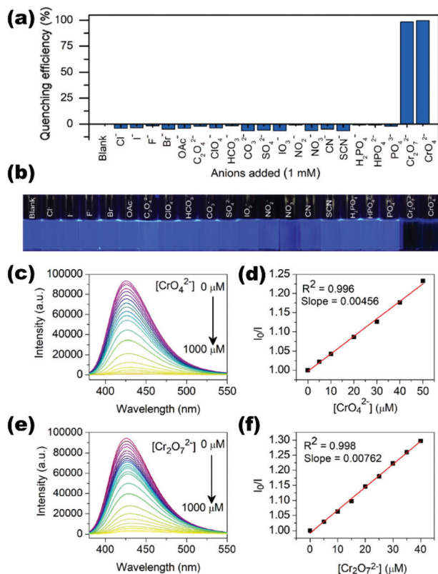
Fig. 14 (a) Quenching percentage of (50) dispersed in different anion solutions; (b) digital images of (50) dispersed in different anion solutions under UV irradiation; (c) and (e) fluorescence spectra of (50) at different concentrations of chromate anion solutions; (d) and (f) linear fitting of the Stern–Volmer plot for (50) in the presence of chromate anions. Reproduced with permission from ref. 95. Copyright 2019 Elsevier B.V.
