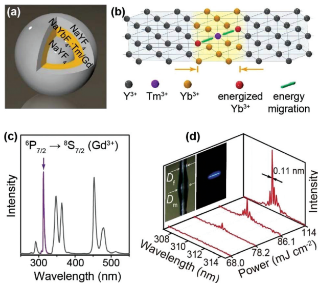
Fig. 8 Yb-Based UCNP for upconversion lasing. (a) Schematic design of sandwich-structured \beta\text{-NaYF}_4@(\text{NaYbF}_4:\text{Tm}^{3+}/\text{Gd}^{3+}) (1/30 mol%)@ \text{NaYF}_4 UCNP. (b) Schematic illustration of energy transfer from \text{Yb}^{3+} to \text{Tm}^{3+} in the Yb-sublattice. (c) Emission spectrum of the \beta\text{-NaYF}_4@(\text{NaYbF}_4:\text{Tm}^{3+}/\text{Gd}^{3+}) (1/30 mol%)@ \text{NaYF}_4 UCNP under 980 nm excitation. (d) Lasing spectra of the micro-resonator containing the \beta\text{-NaYF}_4@(\text{NaYbF}_4:\text{Tm}^{3+}/\text{Gd}^{3+}) (1/30 mol%)@ \text{NaYF}_4 UCNP as gain media under excitation of 980 nm at different power densities. Insets: Photographs of the micro-resonator without and with optical excitation. D_f and D_m denote diameters of the support fibre and microcavity, respectively. Reprinted with permission from ref. 28. Copyright 2016 Springer Nature.
