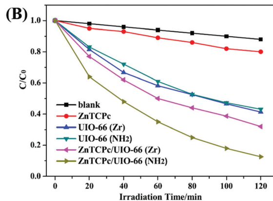
Fig. 18 (A) Proposed mechanism for the degradation of MB by ZnTCPc/UiO-66( NH_2 ) under visible light; (B) degradation dynamics of MB by different samples. Adapted with permission from ref. 124, © 2016 Elsevier B.V.
