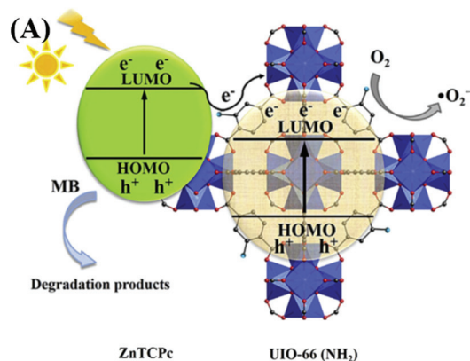
Fig. 18 (A) Proposed mechanism for the degradation of MB by ZnTCPc/UiO-66( NH_2 ) under visible light; (B) degradation dynamics of MB by different samples. Adapted with permission from ref. 124, © 2016 Elsevier B.V.
