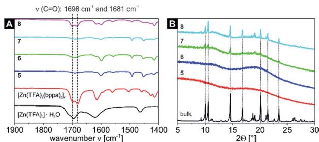
Fig. 3 Detailed view on the spectral range of 1900 cm -1 to 1400 cm -1 of the IR spectra of the starting material [Zn(TFA) 2 ] 2 ·H 2 O, the CN [Zn(TFA) 2 (bppa) 2 ] n and the four [Zn(TFA) 2 (bppa) 2 ] n nanocomposite samples 5–8 (A). The complete spectra can be found in Fig. S8†. Comparison of the PXRD patterns of the bulk material [Zn(TFA) 2 (bppa) 2 ] n and the [Zn(TFA) 2 (bppa) 2 ] n nanocomposite samples 5–8 (B). Most intense PXRD reflexes that correlate with the bulk material are marked with a dashed line.
