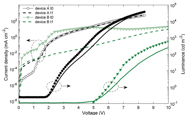
Fig. 3 JVL characteristics of encapsulated top-emitting OLEDs after fabrication (t0) and after seven months (t1). The samples were stored under ambient conditions. Device A has the following stack: glass/Ag/ZnO/TPBi:PEIE/SY/MoO x /Ag/MoO x with evaporated Ag electrodes. Device B corresponds to the all solution-processed OLED, for which the electrodes are replaced by an ink-jet printed Ag layer on PET and a spin-coated WO x / Clevios F HC layer.
