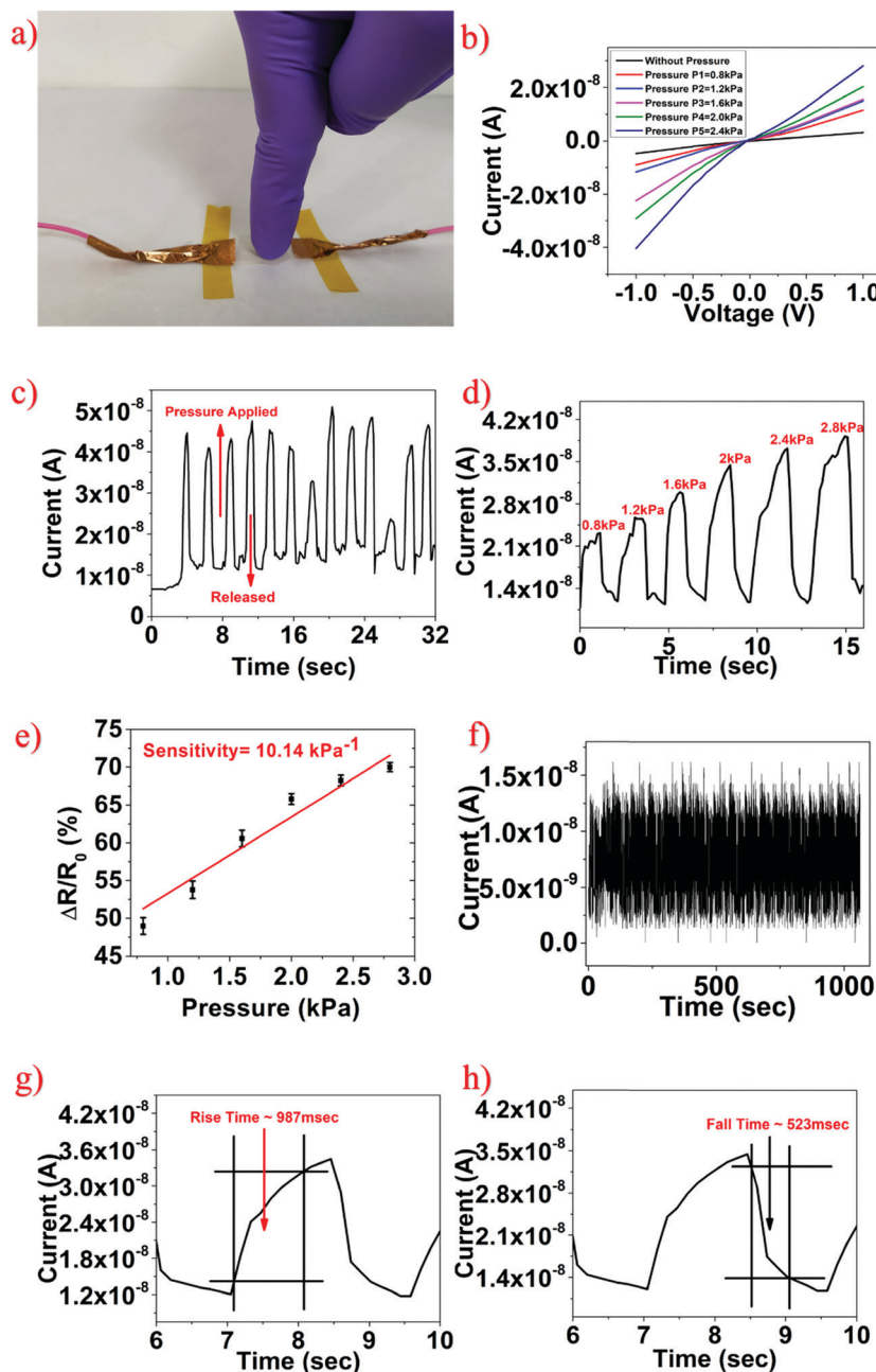
Fig. 7 (a) The digital photo of a finger touching the pressure sensor. (b) I - V characteristics of a SnS 2 QD/PVA based pressure sensor with different applied pressures. (c) Temporal response of the fabricated sensor under constant pressure. (d) Temporal response of the fabricated sensor under different applied pressures. (e) Sensitivity graph showing a sensitivity value of \sim 10.14 \text{ kPa}^{-1} . (f) The response of the fabricated sensor for 1000 cycles. (g and h) The rise time and fall time of the fabricated sensor were \sim 987 \text{ ms} and \sim 523 \text{ ms} .
