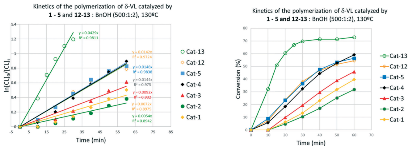
Fig. 11 Left: Plot of \ln[VL]_0/[VL]_t vs. time using complexes 1–5 and 12–13; right: relationship between conversion and time for the polymerization of \delta -VL.
