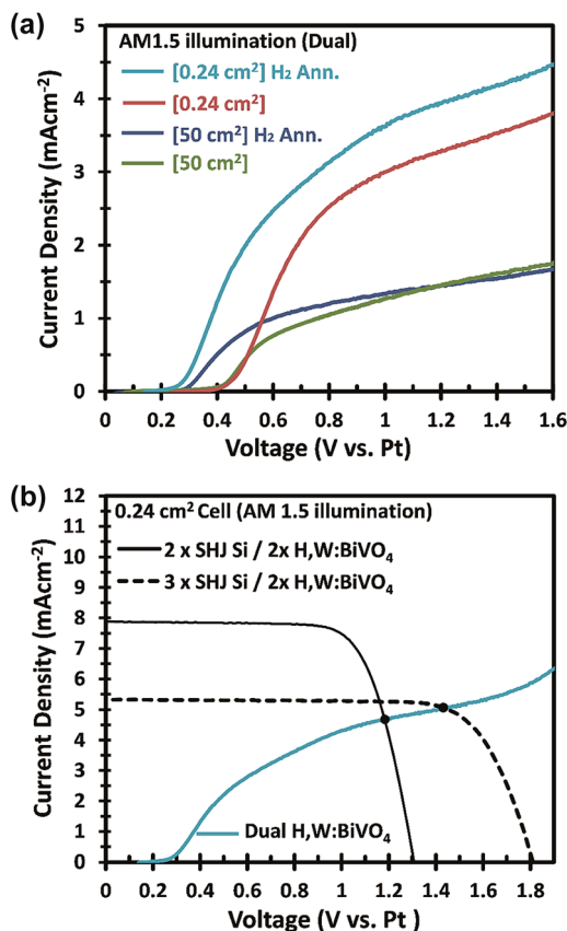
Fig. 9 (a) J - V curves comparing the effects of hydrogen annealing on the small and large area dual- \text{CoPi}/\text{W}:\text{BiVO}_4 photoanodes in 0.1 M \text{KP}_i (small area) or 2.0 M \text{KP}_i (large area) buffer. Large area samples are with Ni lines. (b) J - V curves of a small area 2 SHJ PV (black line) and the 3 SHJ PV (dashed black line) with dual- \text{CoPi}/\text{H},\text{W}:\text{BiVO}_4 photoanodes as the front windows, and the small area dual- \text{CoPi}/\text{H},\text{W}:\text{BiVO}_4 photoanode, measured in 0.1 M \text{KP}_i buffer.
