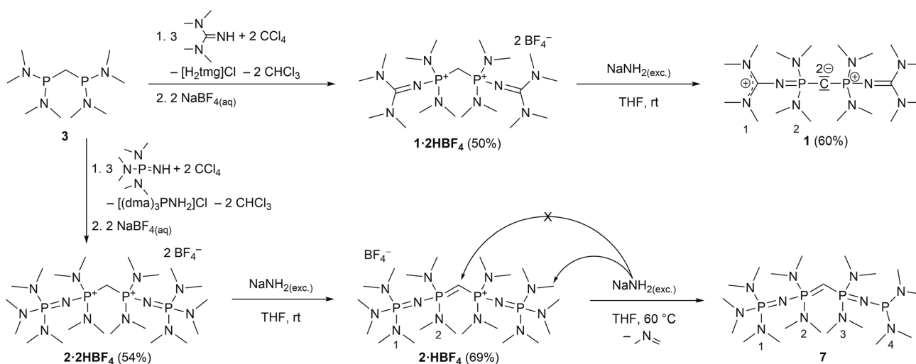
Scheme 1 Preparation of CDP precursors 1 ·2HBF 4 and 2 ·2HBF 4 together with subsequent deprotonation to 1 (one exemplary mesomeric structure displayed) and 7 , respectively. Numbering schemes refer to assigned NMR signals in the experimental section.
