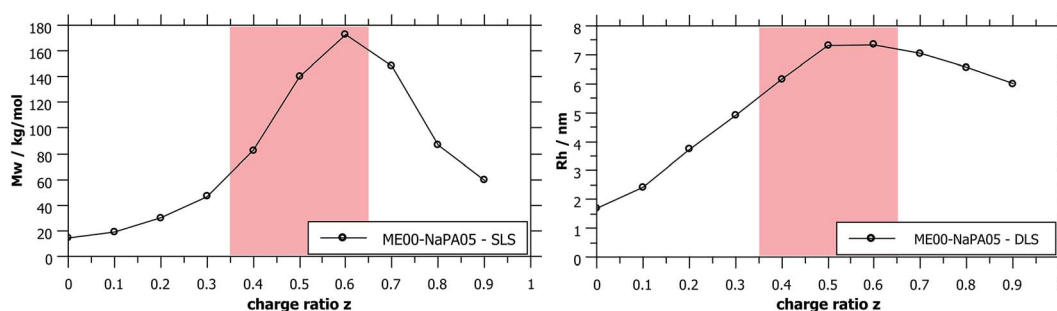
Fig. 3 Apparent M_w and R_h obtained from static and dynamic light scattering show the presence of differently sized aggregates of ME and PE depending on the charge ratio z . Metastable samples (shaded in red) were measured while still being homogeneous, typically being 3–5 days old. Measured values for longer NaPAs are given in Fig. S4.†
