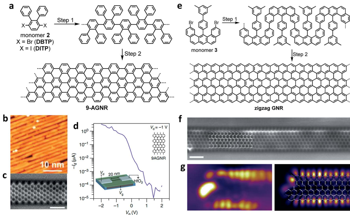
Fig. 3 On-surface syntheses of GNRs under UHV conditions. (a) Synthetic route towards 9-AGNR from monomer 2. (b) STM images showing the length of the 9-AGNR obtained from DITP. Reproduced with permission. 94 Copyright (2018) American Chemical Society. (c) High-resolution noncontact atomic force microscopy (nc-AFM) frequency shift image of 9-AGNR using a CO-functionalized tip. Reproduced with permission. 111 Copyright (2017) American Chemical Society. (d) I_D - V_g of the FET devices showing high I_{on} ( >1 μA) for a 0.95 nm wide 9-AGNR and high I_{on}/I_{off} ( \sim 10^5 ). Inset: scaled 9-AGNR FET schematic. (e) Synthetic route towards a full zigzag GNR from umbrella-shaped monomer 3. (f) Constant height nc-AFM frequency shift image of ZGNR taken with a CO-functionalized tip. (g) Differential conductance maps of filled edge states taken at a sample bias of -0.3 V (left), and density functional theory (DFT)-based local density of states (DOS) at a tip-sample distance of 4 Å, showing the spatial distribution of filled edge states (right). All scale bars are 1 nm. (f and g) Reproduced with permission. 21 Copyright 2016, Macmillan Publishers Ltd.
