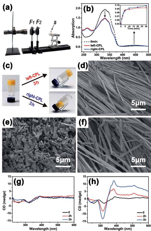
Fig. 2 (a) Photo of the CPL pumping system. F1: Glan–Thompson prism; F2: quarter-wave plate; s: gelator sample. (b) UV-vis spectra of Azo-DF in chloroform ( 0.05 \text{ mg ml}^{-1} ) before (dotted line) and after (solid lines) CPL illumination for 30 min. (c) Gel–sol transition of Azo-DF in chloroform/methanol ( v/v = 1 : 3 , 2 \text{ mg ml}^{-1} ), the gel collapsed under right-CPL irradiation, compared to only few solvent squeezing out from the gel under left-CPL irradiation. (d–f) Scanning electronic microscopy (SEM) images of Azo-DF xerogel before (d) and after 3 h irradiation of right-CPL (e) or left-CPL (f). (g and h) Circular dichroism (CD) spectra of Azo-DF gel in chloroform/methanol ( v/v = 1 : 3 , 2 \text{ mg ml}^{-1} ) before and after the irradiation of right-(g) or left-CPL (h). ( \lambda : 365 \text{ nm} , 5 \text{ mW cm}^{-2} ).
