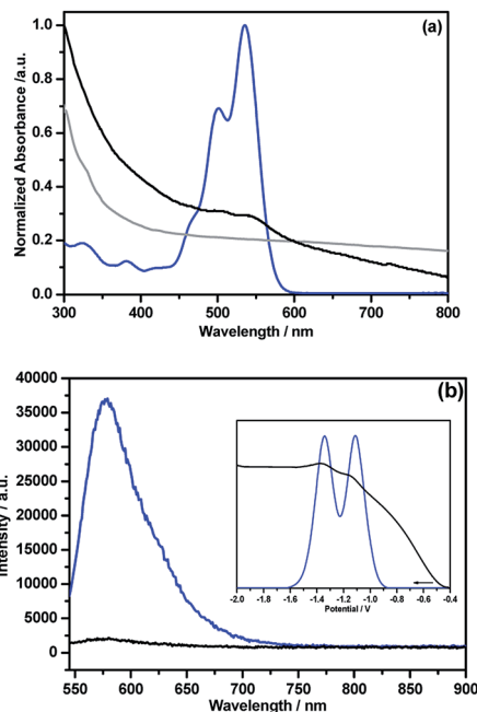
Fig. 5 (a) Absorption and (b) fluorescence ( \lambda_{\text{exc}} = 535 nm) spectra of NG (grey), NG-PDI 1 (black) and PDI 5 (blue) in DCB. (b) Inset shows DPVs of 5 (blue) and 1 (black) in DCB/acetonitrile containing 0.1 M (TBA)ClO 4 .
