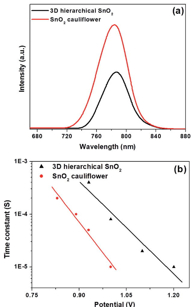
Fig. 8 (a) Steady-state PL spectra of perovskites on different SnO 2 nanostructures and (b) electron lifetime for the perovskites based on different SnO 2 nanostructures.
