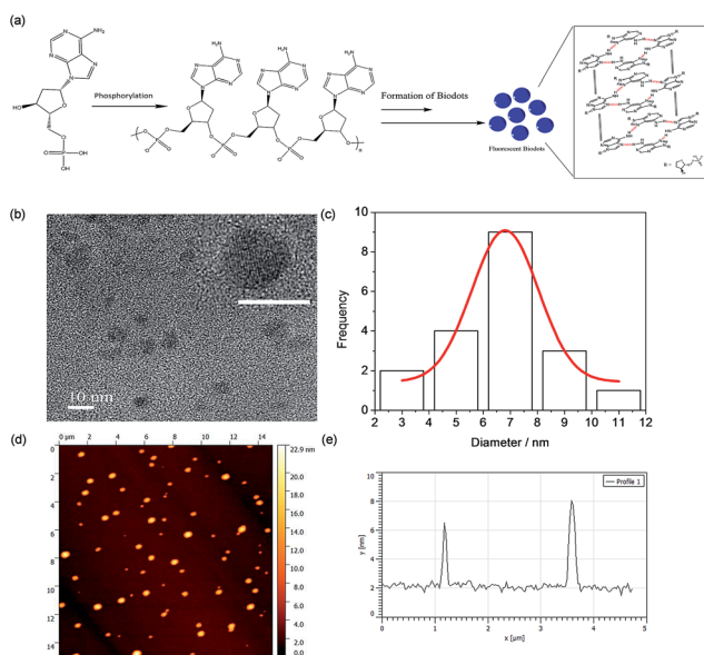
Fig. 5 (a) Proposed formation mechanism of dAMP-dots. (b) TEM image of dAMP-dots; inset shows the HRTEM image with a clear lattice (scale bar represents 10 nm). (c) Size distribution of dAMP-dots. (d) AFM image of dAMP-dots on mica. (e) Height profile of dAMP-dots.
