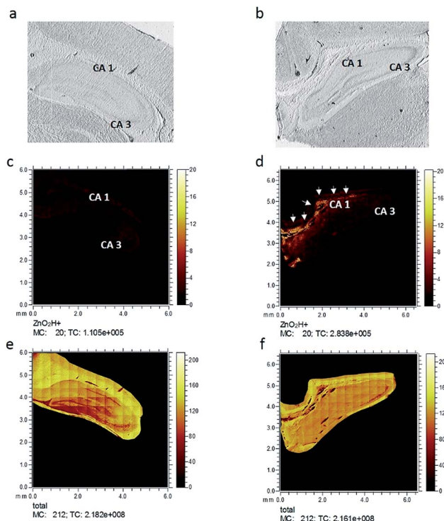
Fig. 2 Optical microscopy images of freeze-dried rat hippocampus sections in (a) control and (b) traumatic brain injured rats. ToF-SIMS ion images showing the spatial signal intensity distribution from [ZnO_2H]^+ species in (c) control and (d) traumatic brain injured rats and for total ion image in (e) control and (f) traumatic brain injured rats across an analysis area of 6 \times 6 mm covering the complete tissue. MC stands for maximum count and TC stands for total count. All data were acquired using a 25 keV Bi_5^+ beam with a maximum primary ion dose of 1.5 \times 10^{11} ions per cm^2 .
