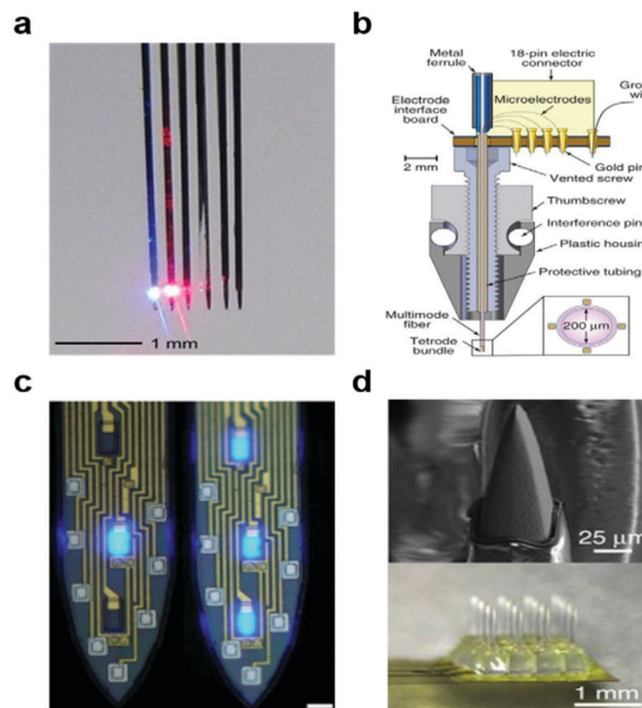
Fig. 9 Optoelectronic neural devices. (a) Multidiode arrays integrated with silicon microelectrodes. Reproduced with permission from ref. 152. Copyright 2012 American Physiological Society. (b) Optrode with combination of ferrule and Ni/Cr based tetrode bundles. Reproduced with permission from ref. 158. Copyright 2012 Nature Publishing Group. (c) Monolithically integrated \mu\text{LED} on silicon neural probe. Reproduced with permission from ref. 164. Copyright 2015 Cell Press. (d) ZnO MOA device for multichannel intracortical neural recording and optical stimulation. Reproduced with permission from ref. 165. Copyright 2015 Nature Publishing Group.
