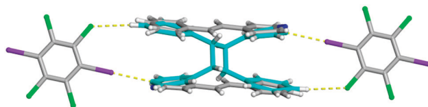
Fig. 4 X-ray structure of the partially photoreacted co-crystal of form I forming the ht-PP shown in turquoise. The I\cdots N halogen bonds and C-H\cdots Cl contacts are shown with yellow dashed lines.
