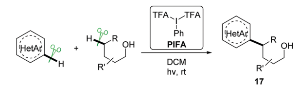
Scope of heteroaryls (reaction with n -pentanol)
