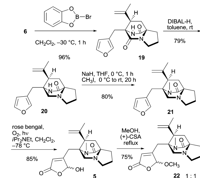
Scheme 4 Synthesis of acetal 22 from tricycle 6 .
