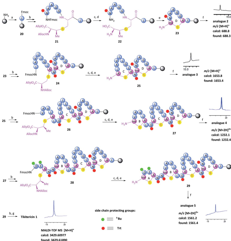
Scheme 3 Fmoc-solid-phase peptide synthesis of tikitericin 1. Reagents and conditions: (a) DIC, Fmoc-Leu-HMPP, CH 2 Cl 2 , 24 h; (b) Fmoc-SPPS: (i) PyBOP, 6-Cl-HOBt, NMM, DMF, 5 min; (ii) 20% piperidine in DMF (v/v), 2 × 5 min; (c) Pd(PPh 3 ) 4 , PhSiH 3 , DMF/CH 2 Cl 2 (v/v, 1/1), 2 h; (d) 20% piperidine in DMF (v/v), 2 × 5 min; (e) PyBOP, 6-Cl-HOBt, NMM, DMF, 2 h; (f) TFA/H 2 O/TIPS (v/v/v, 95/2.5/2.5), 1 h; (g) TFA/H 2 O/TIPS/EDT (v/v/v/v, 94/2.5/2.5/1), 1 h. TIPS, triisopropylsilane; EDT, 1,2-ethanedithiol.
