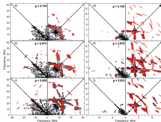
Fig. 5 X-band 4-pulse HYSCORE spectra of [\mathbf{1}\cdot\text{H}_2]^+[\text{BAR}_4^-] (panels (a–c)) and [\mathbf{1}(\text{H}_2)_2]^+[\text{BAR}_4^-] (panels (d–f)) at 2.5 mM in 7 : 1 PhMe : DFB, each collected at three field positions as indicated by g -value. The samples were frozen glasses at 20 K and measured with pulse lengths for ^2\text{H} of \pi/2 = 12 ns and \pi = 8 ns, \tau = 204 ns, initial variable delays of 100 ns and a time step of 20 ns over 300 points in both axes. The pulse lengths for ^1\text{H} were \pi/2 = 8 ns and \pi = 12 ns, \tau = 144, 140, 132 ns (top to bottom), initial variable delays of 100 ns and a time step of 8 ns, and 200 points in both axes. The microwave frequency was 9.7411 and 9.7583 GHz, respectively. Experimental data is in black, while simulations are overlaid in red.
