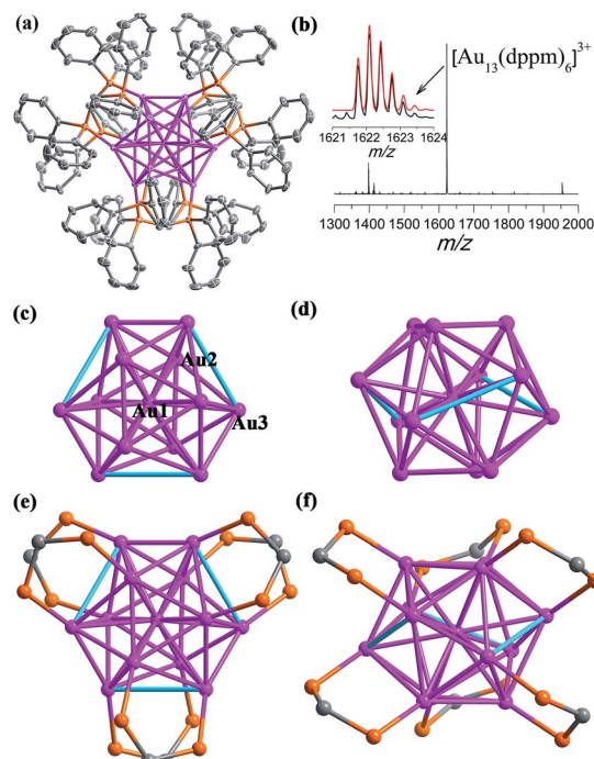
Fig. 1 (a) The X-ray crystal structure of cationic [\text{Au}_{13}(\text{dppm})_6]^{3+} . Thermal contours are drawn at the 50% probability level. Color labels: purple, Au; orange, P; and gray, C. H atoms and \text{Cl}^- ions are omitted. (b) The positive mode of the HRESI-MS of SD/Au1 ·5 Cl dissolved in \text{CH}_2\text{Cl}_2 . Inset: comparison of the measured (black trace) and simulated (red trace) isotopic patterns of [\text{Au}_{13}(\text{dppm})_6]^{3+} . (c and e) Top view of the kernel structure of \text{Au}_{13} along the C_3 axis with the crystallographically unique Au atoms labelled. (d and f) Side view of the kernel structure of \text{Au}_{13} . The three cyan edges denote the longer Au–Au separations (3.4995(5) Å).
