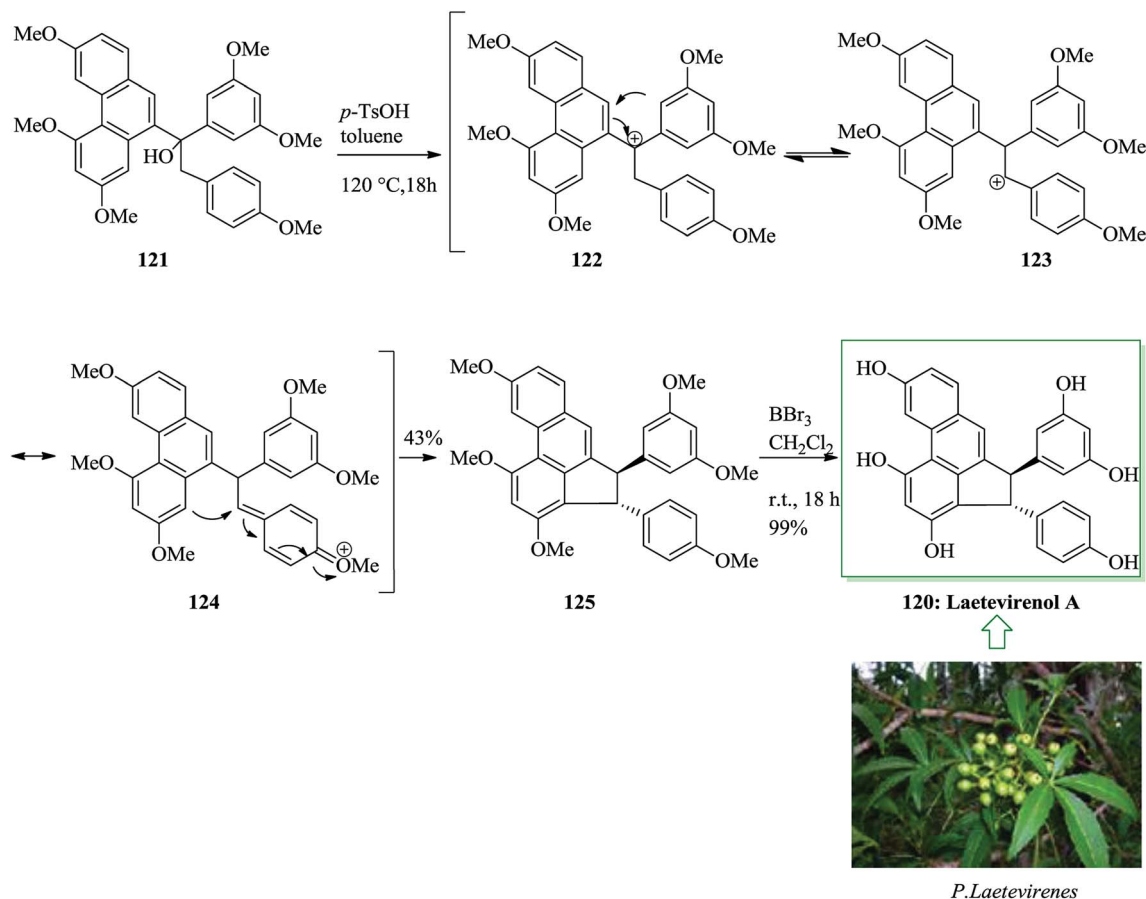
Scheme 26 Total synthesis of laetevireinol A 120.
