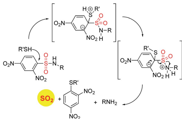
Scheme 7 Thiol activated SO 2 donors.
