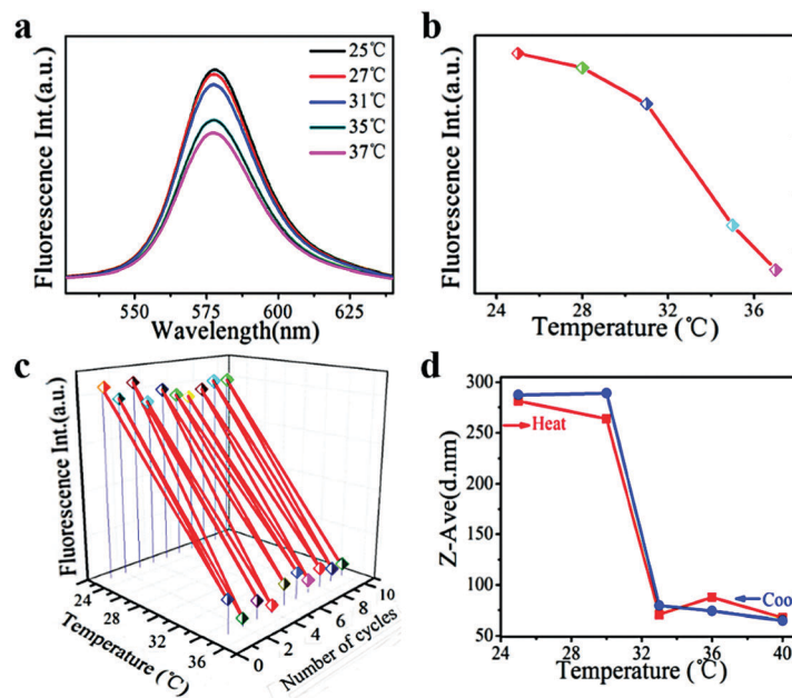
Fig. 7 (a) The fluorescence spectra of Rhodamine B-loaded PNIPAM–FePt at different temperatures. (b) The fluorescence intensity of Rhodamine B-loaded PNIPAM–FePt in water. (c) Alternate heating and cooling experiments of Rhodamine B-loaded PNIPAM–FePt in water between 25 °C (below the LCST) and 37 °C (above the LCST). (d) DLS measurements of Rhodamine B-loaded PNIPAM–FePt in water.
