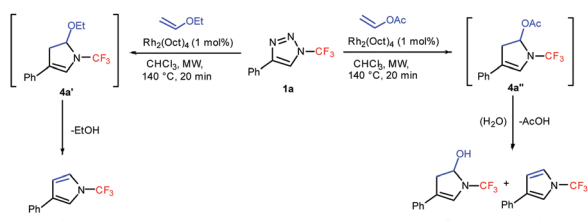
Scheme 2 A comparison of the reactivity of 1a with ethyl vinyl ether and vinyl acetate.
