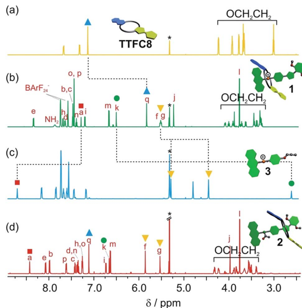
Fig. 3 Stacked partial 1 H NMR spectra (700 MHz, 2 mM, CD 2 Cl 2 , 298 K) of (a) macrocycle TTF C8, (b) charged [2]rotaxane 1 , (c) axle 3 , (d) neutral, acetylated [2]rotaxane 2 . Selected signals are marked with coloured symbols. The solvent residue signal is marked with an asterisk.
