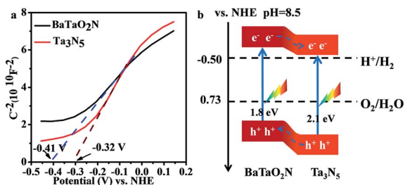
Fig. 4 Band structure characterizations of the \text{Ta}_3\text{N}_5 and BaTaO 2 N samples. (a) Mott-Schottky plot for the \text{Ta}_3\text{N}_5 and BaTaO 2 N electrodes. Electrolyte: 0.5 M \text{Na}_2\text{SO}_4 solution (pH = 8.5, adjusted using NaOH). Frequency: 1000 Hz. (b) The relative band positions of the \text{Ta}_3\text{N}_5/\text{BaTaO}_2\text{N} heterostructure.
