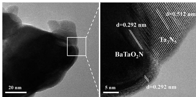
Fig. 3 Representative TEM (left) and locally enlarged HRTEM (right) images of the chosen Ba(0.3)- \text{Ta}_3\text{N}_5 sample.
