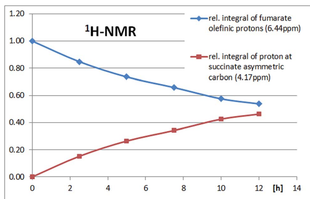
Fig. 5 Timecourse of a biocatalytic Michael addition reaction using a solution of 50 µmol fumarate, 100 µmol L-arginine in 1 mL D 2 O, adjusted to pH 7.5 with NaOH and 20 µL argininosuccinate lyase (ASL) solution (soluble fraction).
