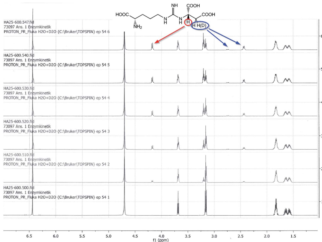
Fig. 4 1 H-NMR of the biocatalytic Michael addition reaction of L-arginine 2 to fumarate 3 in D 2 O. 1 H-NMR signals at 2.75 and 2.43 ppm show a too small integral due to insertion of deuterium from the solvent (D 2 O).
