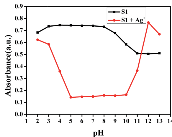
Fig. 5 pH response of S1 and S1-Ag + in the DMSO/ \text{H}_2\text{O} (v:v = 1 : 1; buffered with HEPES) solution.
