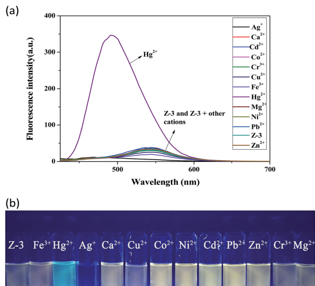
Fig. 1 (a) Fluorescence spectra ( \lambda_{\text{ex}} = 400 \text{ nm} ) of Z-3 ( 2 \times 10^{-5} \text{ M} ) with different metal ions: \text{Fe}^{3+} , \text{Hg}^{2+} , \text{Ag}^{+} , \text{Ca}^{2+} , \text{Cu}^{2+} , \text{Co}^{2+} , \text{Ni}^{2+} , \text{Cd}^{2+} , \text{Pb}^{2+} , \text{Zn}^{2+} , \text{Cr}^{3+} and \text{Mg}^{2+} (10 equiv., respectively) in DMSO/ \text{H}_2\text{O} (v/v, 3 : 2; buffered with HEPES, pH = 7.20). (b) Visual fluorescence emission of the Z-3 sensor upon the addition of different metal ions.
