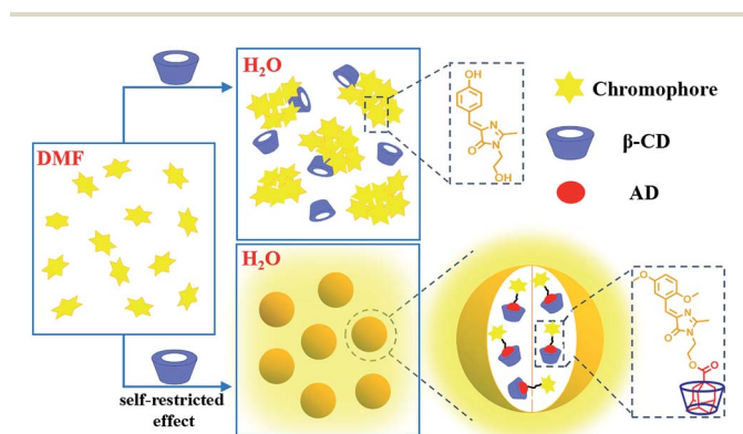
Fig. 1 Concept of emission enhancement of GFP chromophore in aggregated state. Upper: the aggregated emission of GFP chromophore (HBI) is very dim due to free conformational motion and ACQ; below: the aggregated emission is greatly enhanced via self-restricted effect and host-guest interaction.
