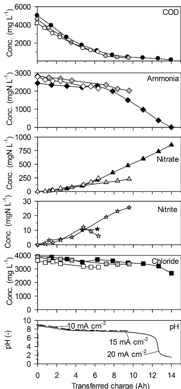
Fig. 1 Galvanostatic electrolysis of high-concentration urine on BDD. Full symbols: 20 mA cm -2 (25.2 °C), grey symbols: 15 mA cm -2 (25.1 °C) and empty symbols 10 mA cm -2 (25.0 °C). Electrode gap: 9 mm.
