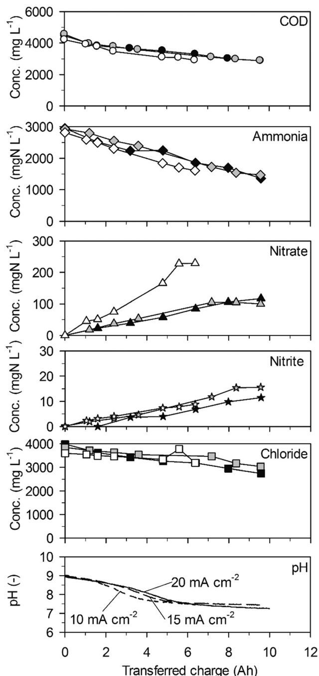
Fig. 2 Galvanostatic electrolysis of high-concentration urine on TDIROF. Full symbols: 20 mA cm -2 (25.1 °C), grey symbols: 15 mA cm -2 (25.0 °C) and empty symbols 10 mA cm -2 (25.0 °C). Electrode gap: 10 mm.
