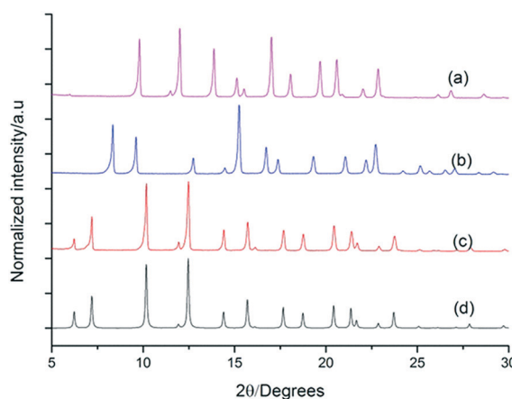
Fig. 4 Experimental PXRD of (a) FT-RCC3- R (space group symmetry, F 4 1 32) (b) racemic CC1 ( R 3), and (c) activated quasiracemate (FT-RCC3- R )-(CC1- S ) ( F 23). All crystallised from CH 2 Cl 2 /acetone. (d) Simulated PXRD of desolvated quasiracemate (FT-RCC3- R )-(CC1- S ).
