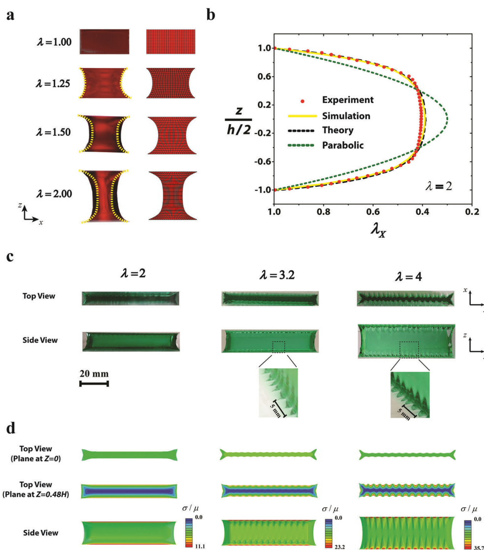
Fig. 3 Experimental, simulation and theoretical results on the deformation and fringe instability in relatively thick layers. (a) Comparison of experimental and simulation results on deformation of a layer with W/H = 2 under various applied stretches prior to the fringe instability. (b) Comparison of experimental, simulation and theoretical results on the meniscus shape of a layer with W/H = 2 at applied stretch \lambda = 2 . (c) Experimental observation of the formation of fringe instability for a layer with W/H = 2 as the applied stretch increases. (d) Numerical simulation of the formation of fringe instability for a layer with W/H = 2 as the applied stretch increases. \bar{\sigma} represents the von Mises stress.
