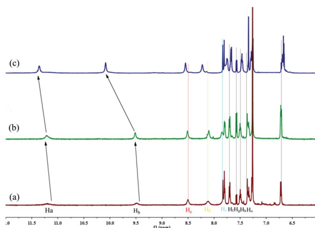
Fig. 2 Partial 1 H NMR spectra of G in CDCl 3 with different concentrations, (a) 10 mg ml -1 ; (b) 20 mg ml -1 ; (c) 30 mg ml -1 .
