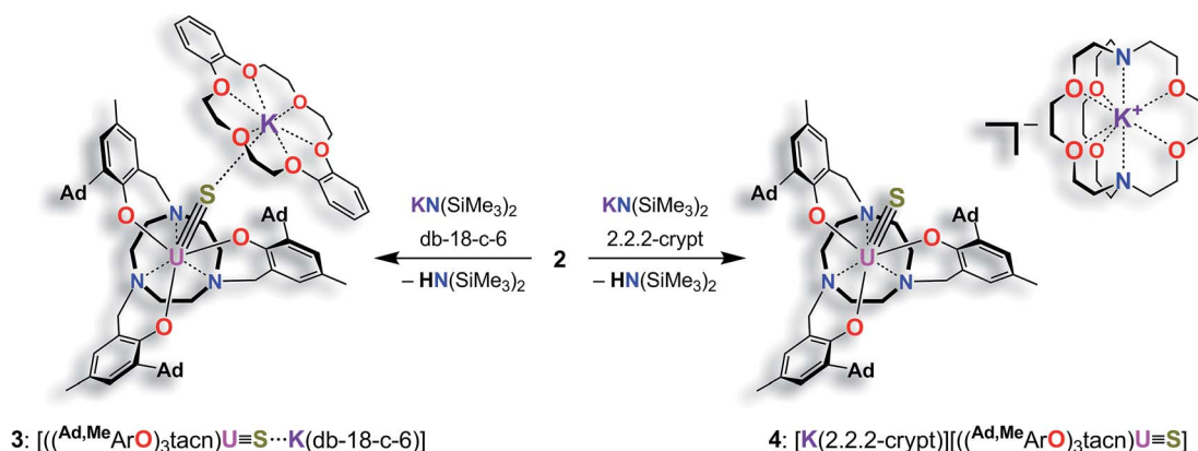
Scheme 2 Synthesis of the terminal uranium(IV) sulfido complexes [((^{\text{Ad,Me}}\text{ArO})_3\text{tacn})\text{U}=\text{S}\cdots\text{K}(\text{db-18-c-6})] ( 3 ) and [\text{K}(2.2.2\text{-crypt})][((^{\text{Ad,Me}}\text{ArO})_3\text{tacn})\text{U}=\text{S}] ( 4 ).
