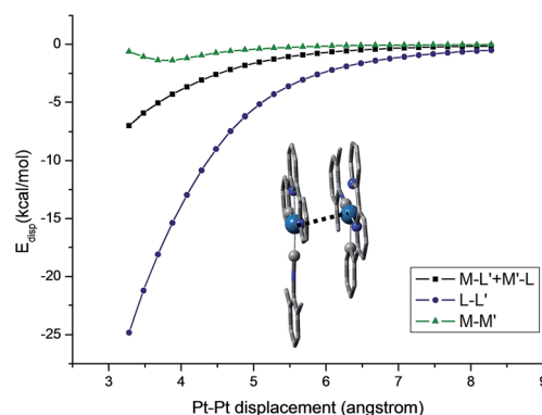
Fig. 13 Dispersion contributions of the metal atoms and ligand fragments to the dimer [61-PF 6 ] 2 2+ . The Pt \cdots Pt' distance was used as a reaction coordinate.
