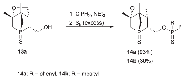
Scheme 5 Synthesis of phosphinites 14 .
