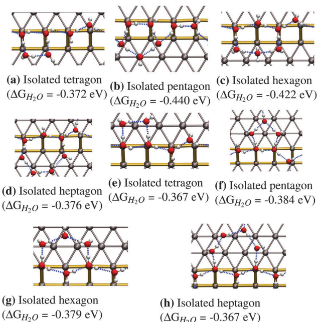
(a) Isolated tetragon ( \Delta G_{H_2O} = -0.372 eV) (b) Isolated pentagon ( \Delta G_{H_2O} = -0.440 eV) (c) Isolated hexagon ( \Delta G_{H_2O} = -0.422 eV) (d) Isolated heptagon ( \Delta G_{H_2O} = -0.376 eV) (e) Isolated tetragon ( \Delta G_{H_2O} = -0.367 eV) (f) Isolated pentagon ( \Delta G_{H_2O} = -0.384 eV) (g) Isolated hexagon ( \Delta G_{H_2O} = -0.379 eV) (h) Isolated heptagon ( \Delta G_{H_2O} = -0.367 eV)
