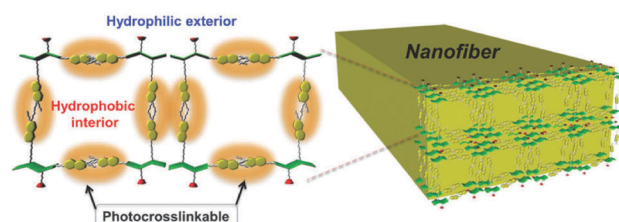
Fig. 15 Diagram showing the possible cross-linking within a fibre due to coumarin dimerisation of the dipeptide functionalised hydrogelator. Reproduced from ref. 106 with permission from the Centre de la Recherche Scientifique (CNRS) and the Royal Society of Chemistry.
