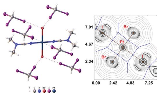
Fig. 2 Left: View of fragment \mathbf{1b}\cdot(\text{CHI}_3)_6 from \mathbf{1b}\cdot 2\text{CHI}_3 . Thermal ellipsoids are shown with 50% probability and short contacts are indicated by dotted lines. Coordinates of this fragment were applied in further DFT calculations. Right: Contour line diagram of the Laplacian distribution \nabla^2\rho(r) (cross-section along the plane \text{Pt-Br-I} ) was received as a result of the topological analysis of the electron density distribution in the model structure. Bond paths are shown as brown lines, selected zero-flux surfaces – as blue lines, bond critical points (3, -1) are shown in blue, nuclear critical points (3, -3) – in pale brown, length unit – Å.
