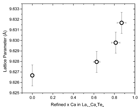
Fig. 3 The lattice parameter of the \text{La}_{3-x}\text{Ca}_x\text{Te}_4 as a function of the refined calcium content. Y-error bars represent the instrumental limit of \pm 0.001 \text{ \AA} and X-error bars represent a 5% uncertainty.
