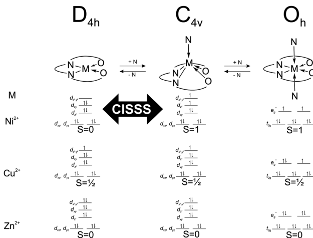
Scheme 2 Electronic configuration, spin number and geometry of the different complexes in equilibrium in solution upon addition of pyridine.
