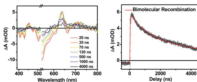
Fig. 7 Nanosecond transient spectra of an annealed film of 1 (left) and its transient kinetic trace at 645 nm (right). The nsTA data (black points) is fit using a bimolecular decay (red line).
