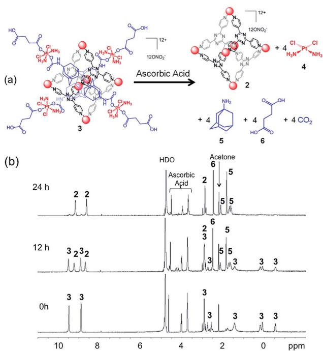
Fig. 2 (a) Chemical representation of the reduction of 3 by ascorbic acid and (b) ^1H NMR (400 MHz, R.T.) spectra showing reduction of 3 ( 0.8 \text{ mM} ) by ascorbic acid ( 8 \text{ mM} ) in deuterated PBS over 24 h at 37^\circ\text{C} .
