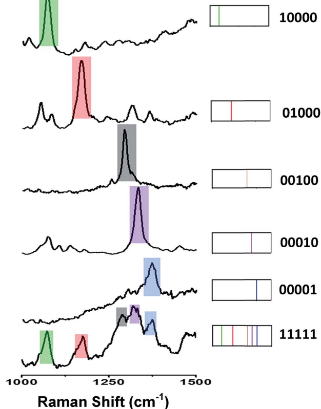
Fig. 4 Typical Raman spectra (left) on microbeads with different types of SERS label using different Raman reporters (10000, 01000, 00100, 00010, 00001 and 11111) and their corresponding spectral barcodes (right).
