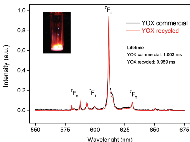
Fig. 12 Luminescence spectra ( \lambda_{\text{exc}} = 254 \text{ nm} ) of the commercial red Y_2O_3:Eu^{3+} (YOX) phosphor, compared with the spectrum of the recycled YOX phosphor after calcination of the (Y,Eu)_2(C_2O_4)_3 precipitate. The spectra were scaled to have the same intensity for the {}^5D_0 \rightarrow {}^7F_1 transition in order to compare the intensity of the hypersensitive {}^5D_0 \rightarrow {}^7F_2 transition. Picture: recycled YOX phosphor in a quartz container irradiated with 254 nm light. The luminescence lifetimes are also shown (Fig. S3†).
